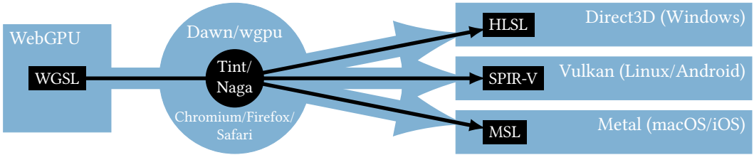
Fig. 2. A block diagram of how the WebGPU API is implemented. Blue relates to APIs and their implementation. Black relates to the languages used within these APIs and their compilation.
